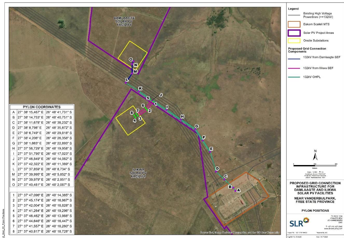
Figure 4: Pylon positions
